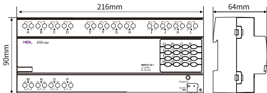
Figure 8. Dimensions - Front View
