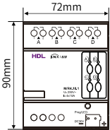
Figure 5. Dimensions - Front View
